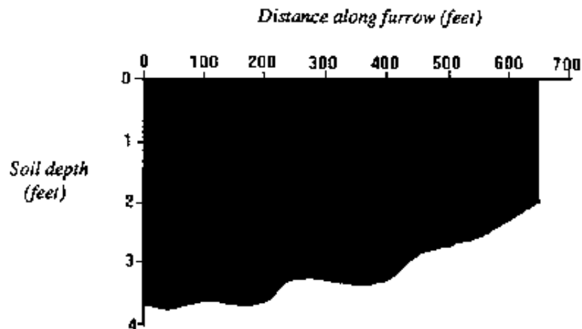
Figure 1. Fertilizer pattern resulting from injecting during entire irrigation.
