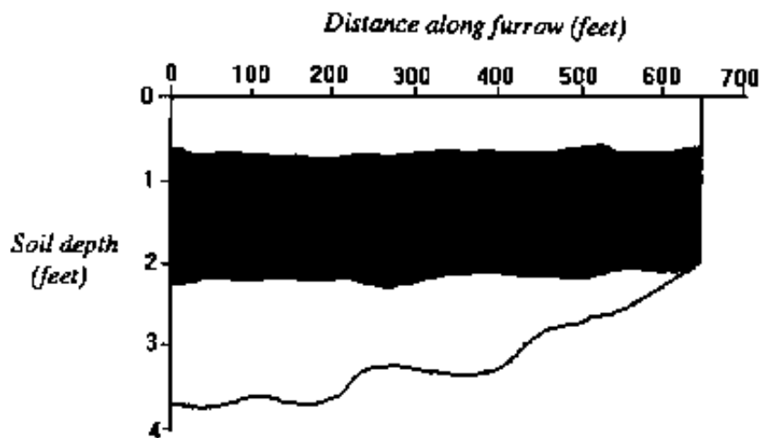
Figure 3. Fertilizer pattern resulting from applying fertilizer during the first part of the surface runoff period.
