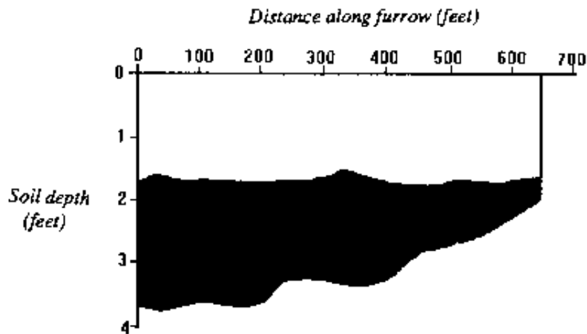
Figure 2. Fertilizer pattern resulting from injecting during the entire water advance period.
