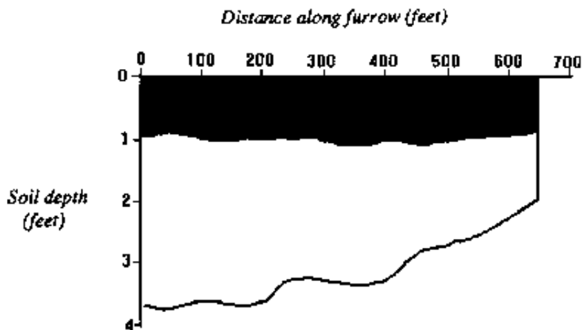
Figure 4. Fertilizer pattern resulting from applying fertilizer during the latter part of the surface runoff period.
